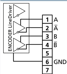
Terminal board X410A
