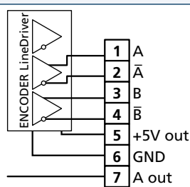
Terminal board X410A
