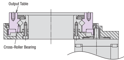
DG85, 130, 200 Structure
