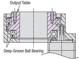
DG85, 130, 200 Structure
