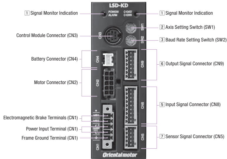
[Driver Top]
