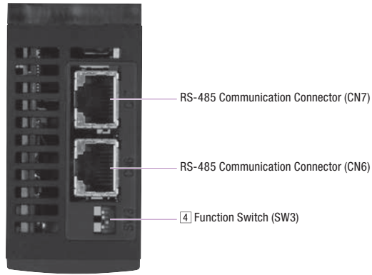
[Driver Top]
