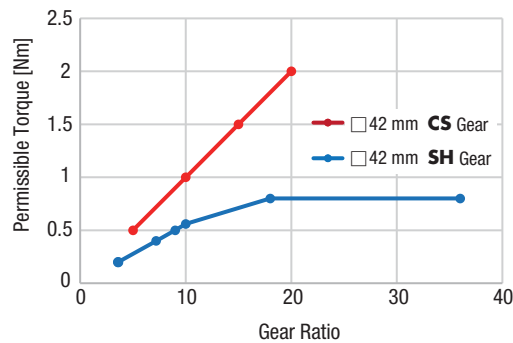
Fig. 13 Permissible Torque Comparison
