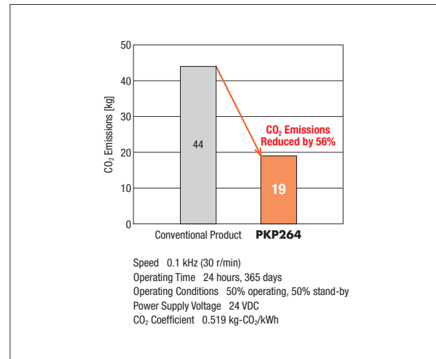
Fig. 4 Reduced Power Consumption and CO 2 Emissions
