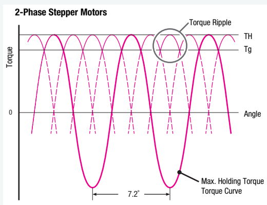
Fig. 2 Angle – Torque Characteristics Ripple (1.8°/step)
