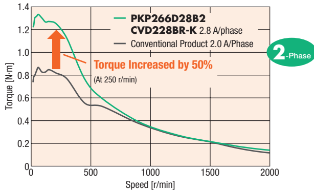
Fig. 7 Speed – Torque Characteristics
