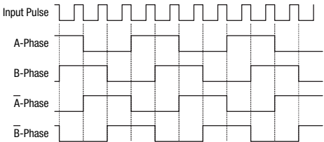
Fig. 5 Sequence Example
