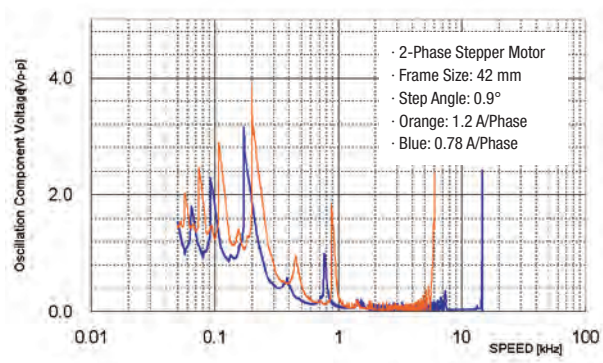
Fig. 6 Drive Current and Vibration Characteristics
