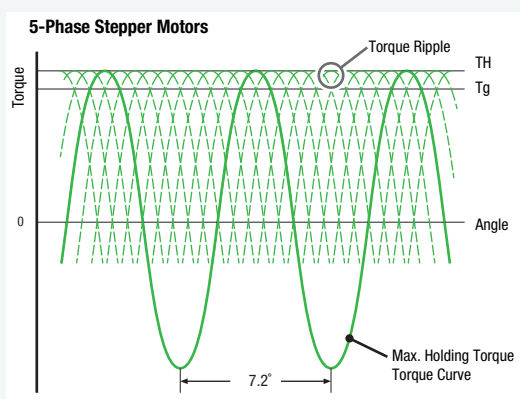
Fig. 3 Angle – Torque Characteristics Ripple (0.72°/step)
