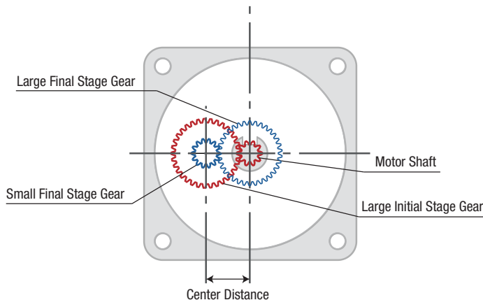
Fig. 10 Concentric Structure of Conventional Parallel Shaft Gear Design (Front)
