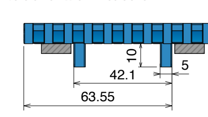
Version C - With 2 Positioner
