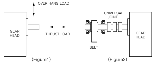
(Table 3) Allowances OVERHANG load and Allowances THRUST load
