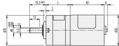
GEARHEAD LENGTH
