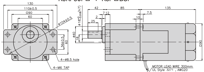
K9RP90F□ + K9P□BUF
