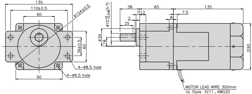
K9RP90F□ + K9P□BF
