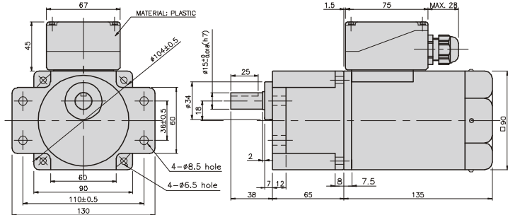
K9RP90F□-T5 + K9P□BF
