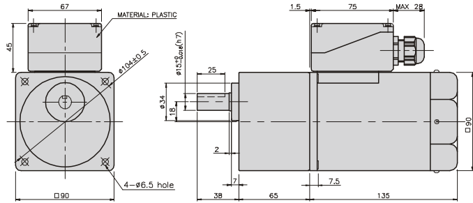
K9RP90F□-T5 + K9P□B
