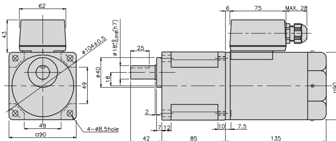
K9RP90F□-T + K9P□BU
