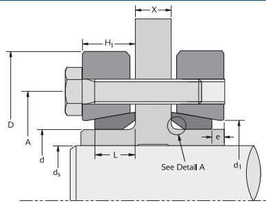
Split Shrink Disc - Type HS
