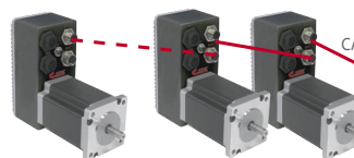
Profibus or DeviceNet Slave
